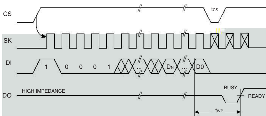
Figure 5-6. WRAL Timing (1)
