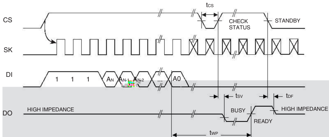
Figure 5-7. ERASE Timing
